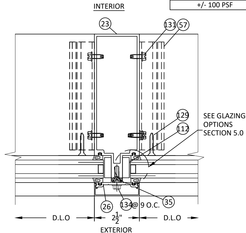
36 HORIZONTAL SECTION 4.2 9" VERTICAL MULLION TUBULAR PROFILE
