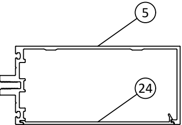
HORIZONTAL MULLION FOR 7-1/2" TUBULAR STANDARD
