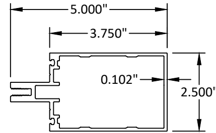
18 VERTICAL/HORIZONTAL FOR 1" GL 6063-T6
