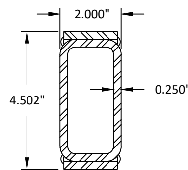
108 STEEL REINFORCEMENT STEEL
