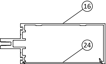
HORIZONTAL MULLION FOR 7-1/2" OPEN BACK STANDARD (LAST BAY)
