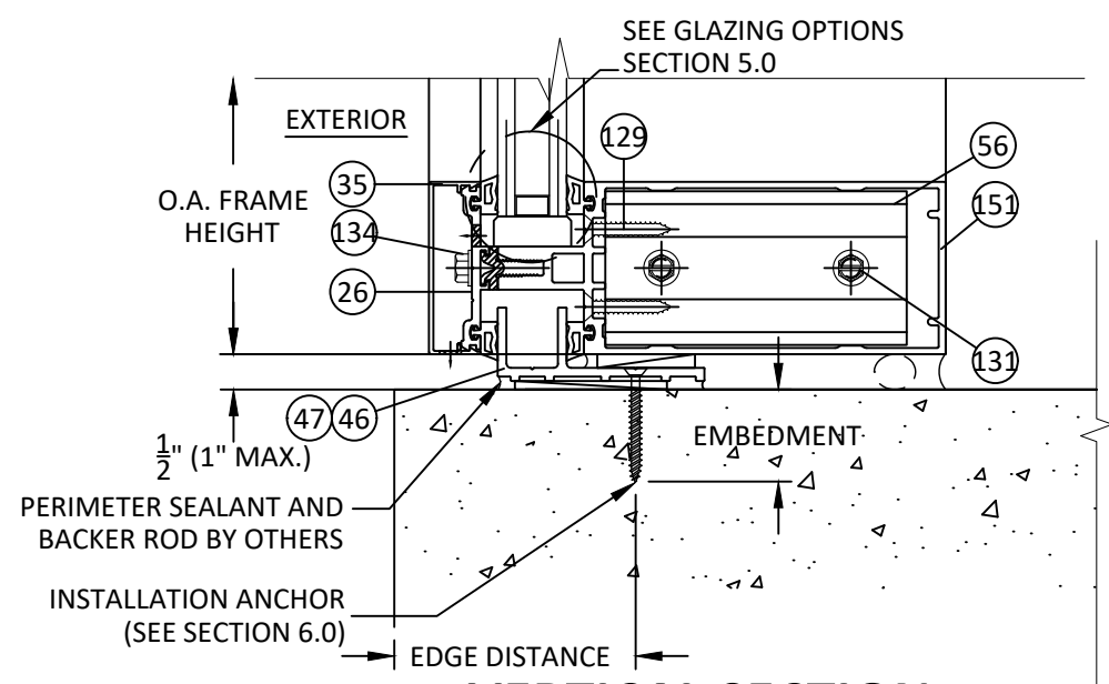
17 3.2 VERTICAL SECTION 7 1/2" SILL - CONCRETE/MASONRY DOUBLE HOLLOW PROFILE ALTERNATE PERIMETER ANCHOR
