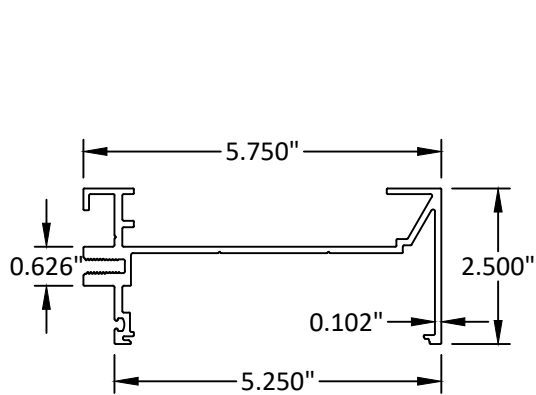
4 INCIDENTAL WATER HEAD FOR 1/4" GL 6063-T5
