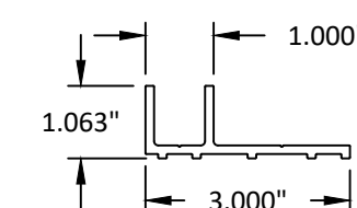
47 PERIMETER ANCHOR 6063-T5
