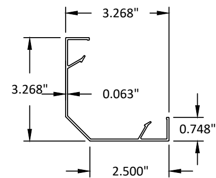
39 90 ° OUTSIDE CORNER FACE COVER 6063-T5
