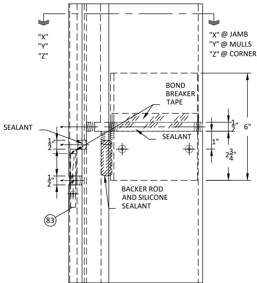
54 6.3 SPLICE SLEEVE VERTICAL DETAIL
