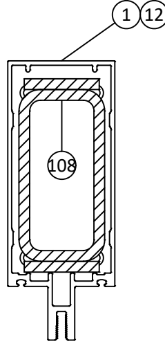
M10 VERTICAL MULLION FOR 7-1/2" STANDARD WITH STEEL REINFORCING
