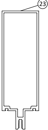
M5 VERTICAL MULLION/JAMB FOR 9" TUBULAR STANDARD
