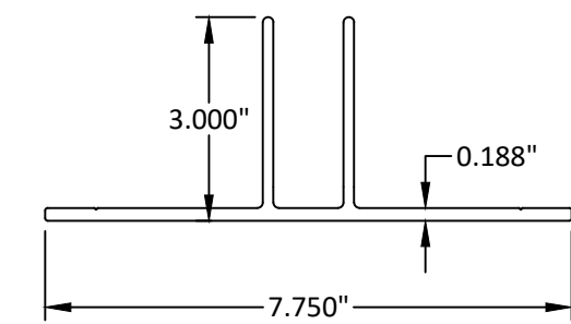
84 MULLION "T" ANCHOR 6063-T5
