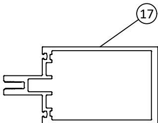
HORIZONTAL MULLION FOR 6" HEAVY DUTY TUBULAR STANDARD
