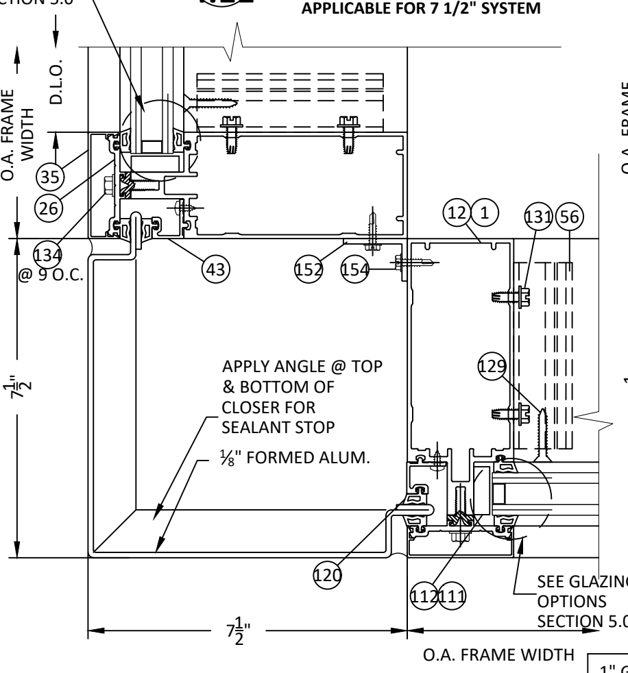
42 HORIZONTAL SECTION 4.11 90 DEG. OUTSIDE CORNER OPTIONAL APPLICABLE FOR 7 1/2" SYSTEM
