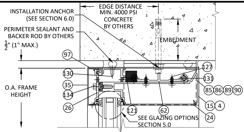
19 3.2 VERTICAL SECTION 7 1/2" HEAD - CONCRETE/MASONRY INCIDENTAL WATER HEAD DETAIL
