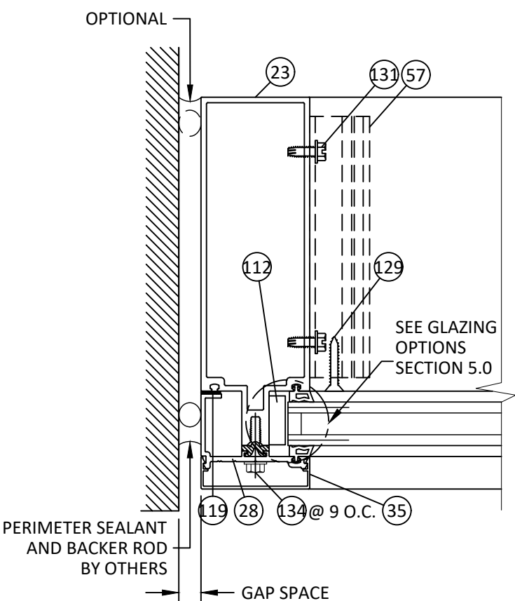
35 HORIZONTAL SECTION 4.2 9" JAMB MULLION TUBULAR PROFILE
