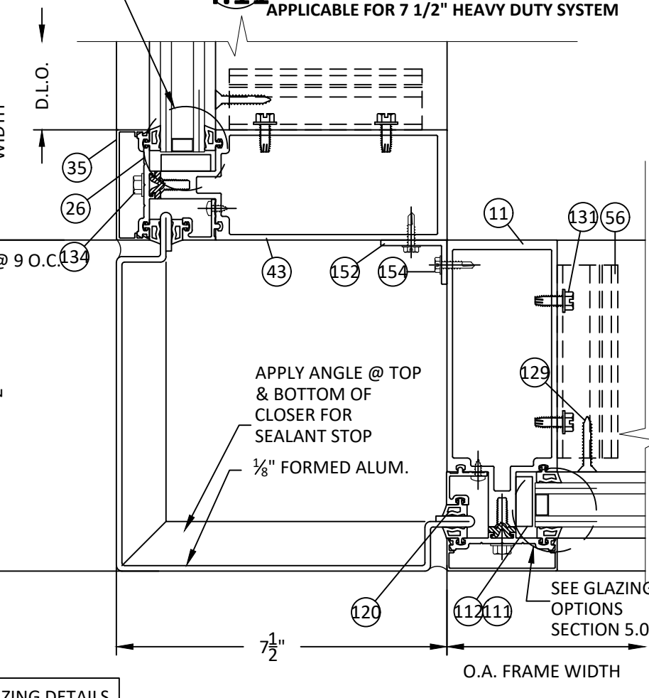
43 HORIZONTAL SECTION 4.11 90 DEG. OUTSIDE CORNER OPTIONAL APPLICABLE FOR 7 1/2" HEAVY DUTY SYSTEM
