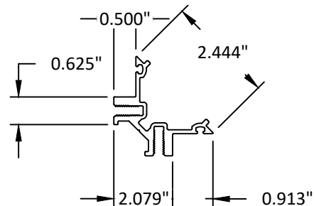
31 90° OUTSIDE CORNER ADAPTOR 6063-T5
