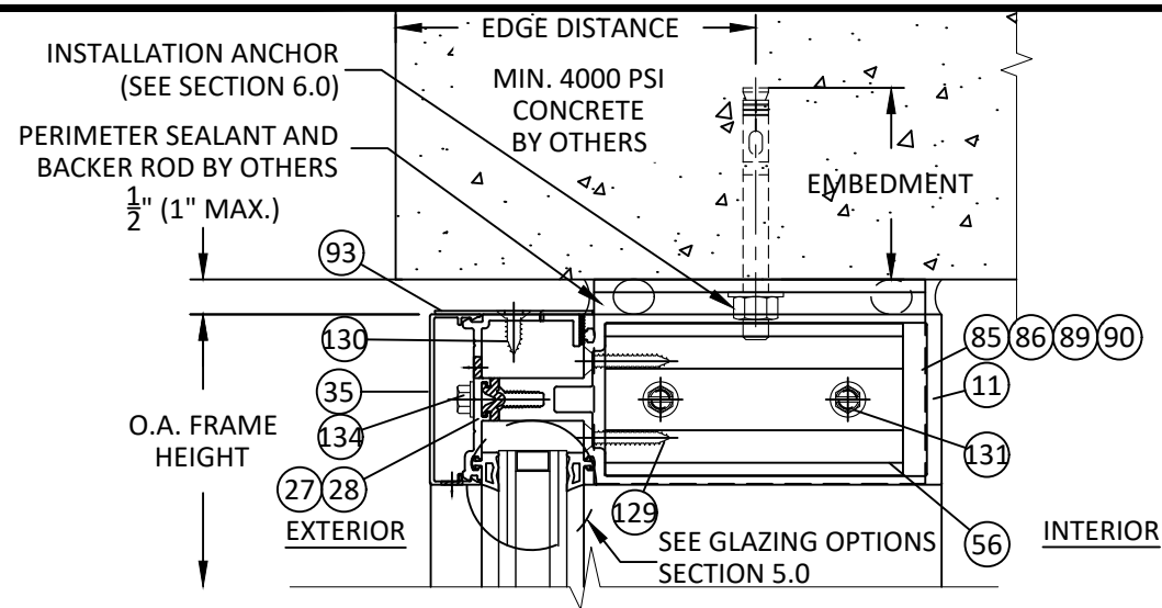
16 3.2 VERTICAL SECTION 7 1/2" HEAVY DUTY HEAD - CONCRETE/ MASONRY HD TUBULAR PROFILE
