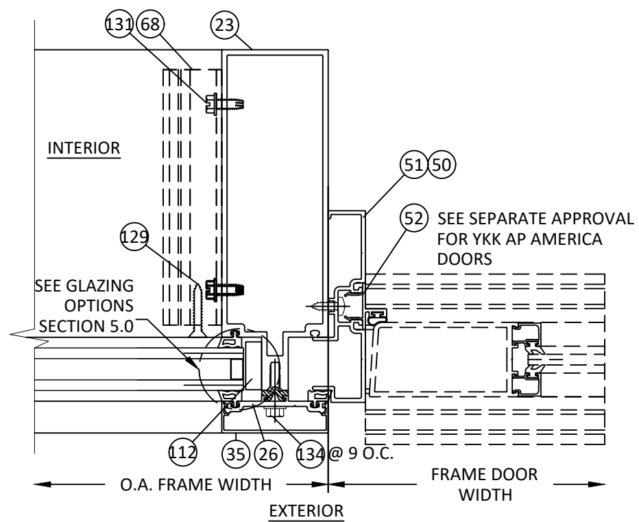
37 HORIZONTAL SECTION 4.2 9" DOOR JAMB MULLION STANDARD PROFILE
