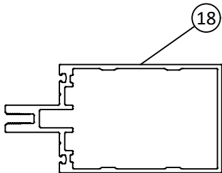
HORIZONTAL MULLION FOR 6" TUBULAR STANDARD
