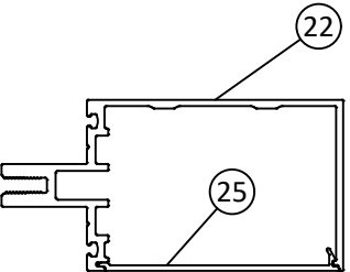
HORIZONTAL MULLION FOR 6" OPEN BACK STANDARD (LAST BAY)
