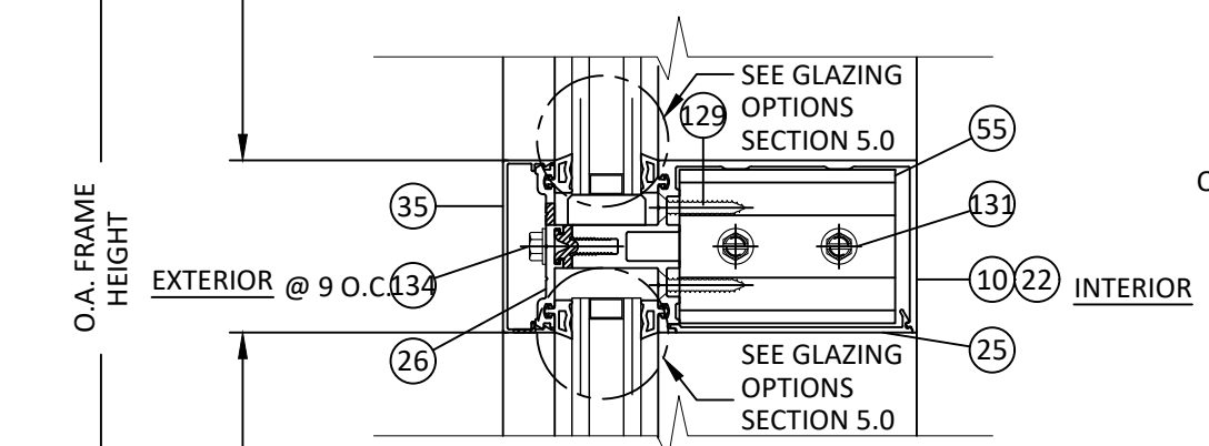
2 3.0 VERTICAL SECTION 6" HORIZONTAL MULLION OPEN BACK PROFILE, LAST BAY
