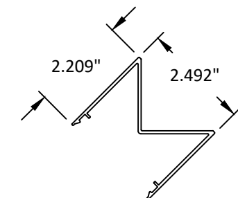
41 90 ° OUTSIDE CORNER INT. COVER 6063-T5
