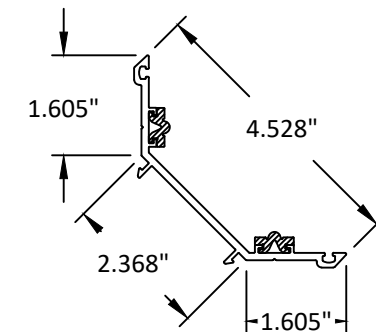
34 90° OUTSIDE CORNER PRESSURE PLATE 6063-T5
