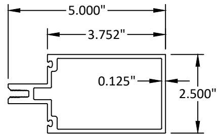
17 HD VERTICAL/HORIZONTAL FOR 1" GL 6063-T5
