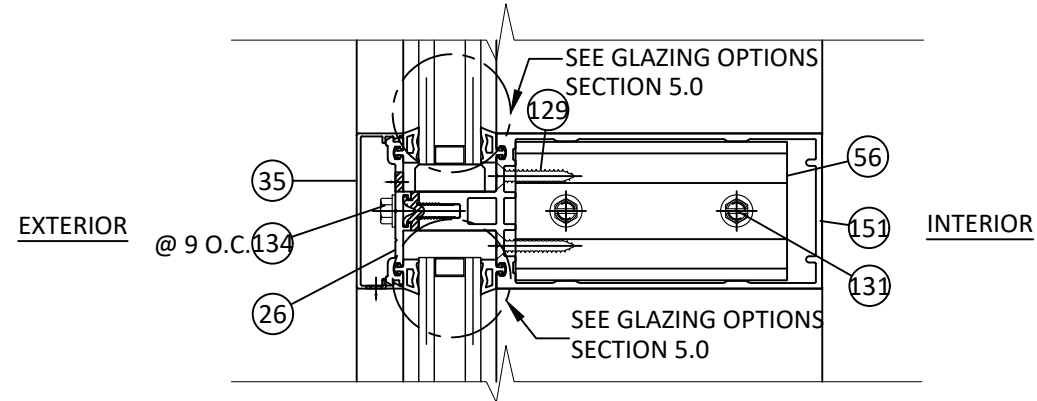
18 3.2 VERTICAL SECTION 7 1/2" HORIZONTAL MULLION DOUBLE HOLLOW PROFILE
