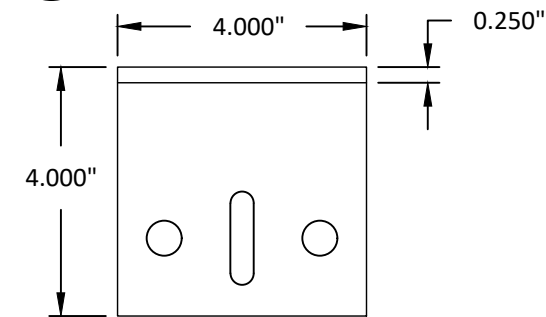
104 WIND LOAD ACHOR STEEL
