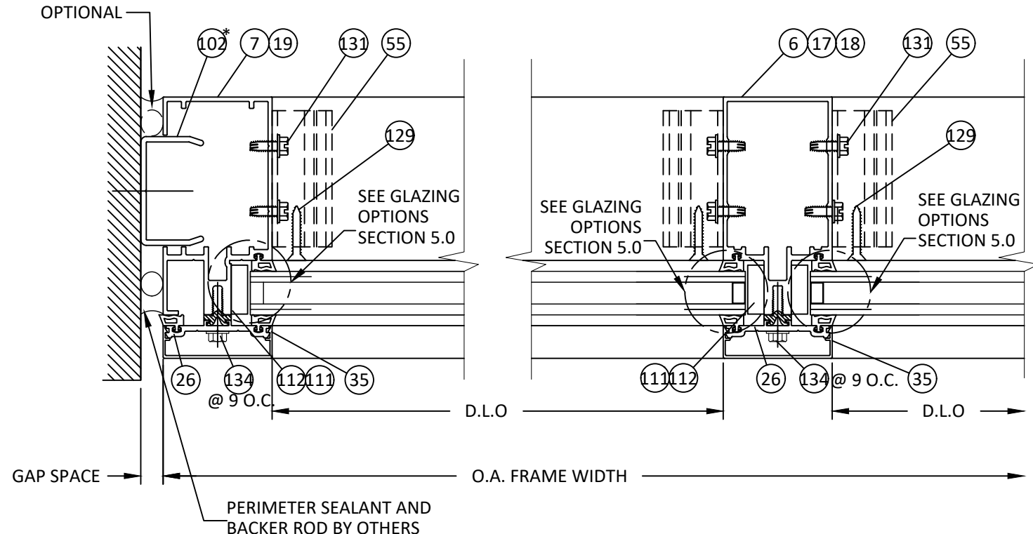
23 4.0 HORIZONTAL SECTION 6" JAMB MULLION OPEN BACK PROFILE W/ OPTIONAL ANCHOR
