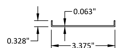
83 FACE COVER SPLICE SLEEVE 6063-T5
