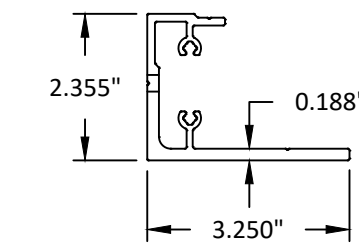
58 "J" ANCHOR 6063-T5
