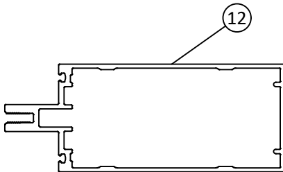
HORIZONTAL MULLION FOR 7-1/2" TUBULAR STANDARD
