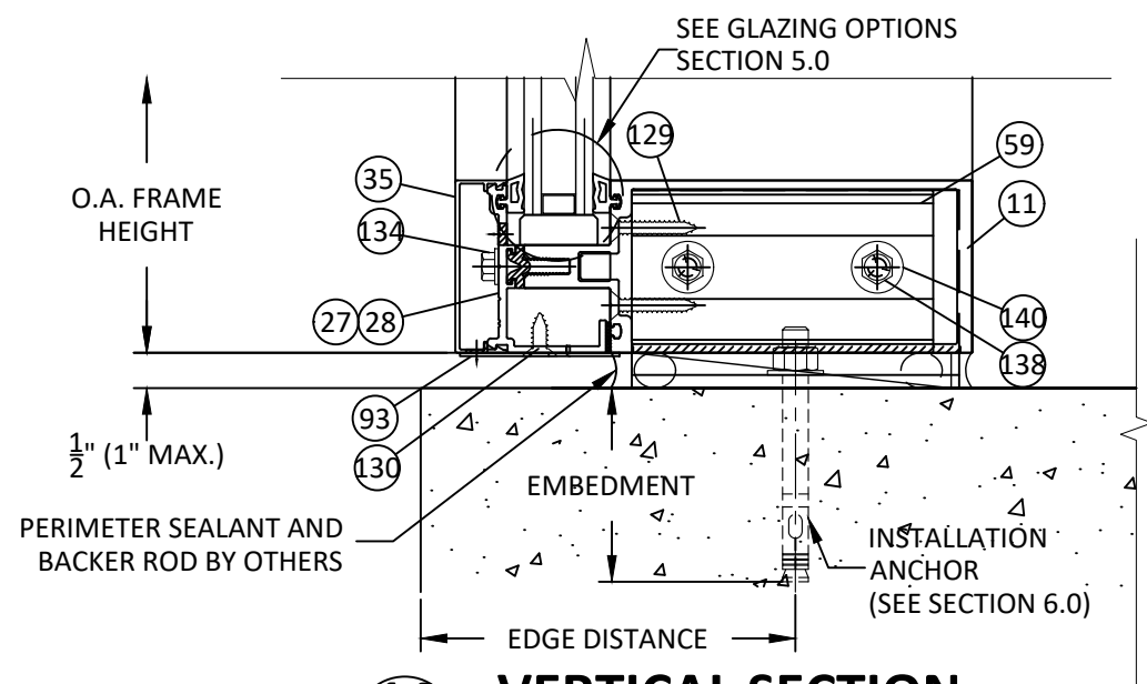
14 3.2 VERTICAL SECTION 7 1/2" HEAVY DUTY SILL - CONCRETE/MASONRY HD TUBULAR PROFILE OPTIONAL "J" ANCHOR
