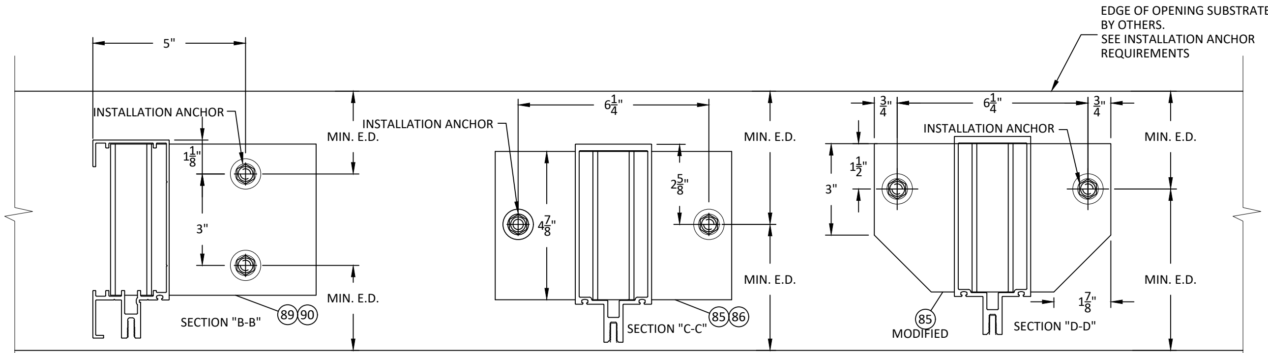
48 6.1 HORIZONTAL SECTION F-ANCHOR 7 1/2" SYSTEM
