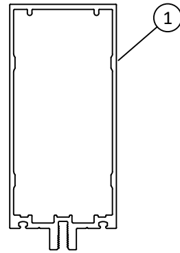
M4 VERTICAL MULLION/ JAMB FOR 7-1/2" HEAVY DUTY TUBULAR OPTION
