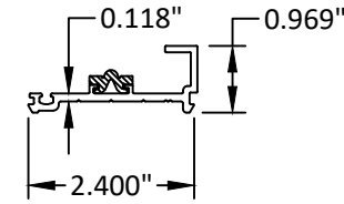
27 PRESSURE PLATE 6063-T5
