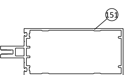
HORIZONTAL MULLION FOR 7-1/2" DOUBLE HOLLOW OPTION
