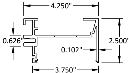
9 INCIDENTAL WATER HEAD FOR 1/4" GL 6063-T5
