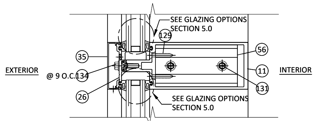
15 3.2 VERTICAL SECTION 7 1/2" HEAVY DUTY HORIZONTAL MULLION HD TUBULAR PROFILE
