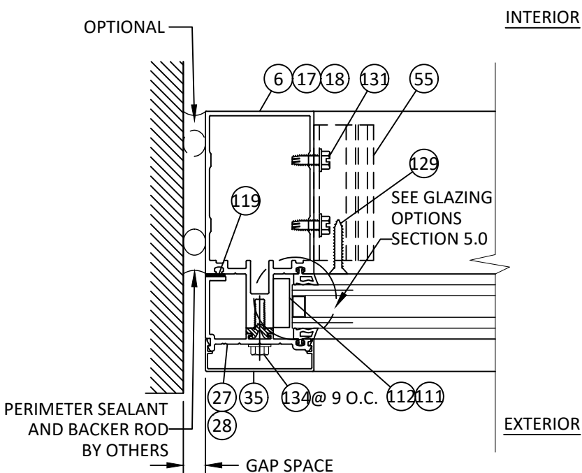
26 4.0 HORIZONTAL SECTION 6" JAMB MULLION TUBULAR PROFILE
