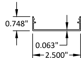
35 3/4" FACE COVER 6063-T5
