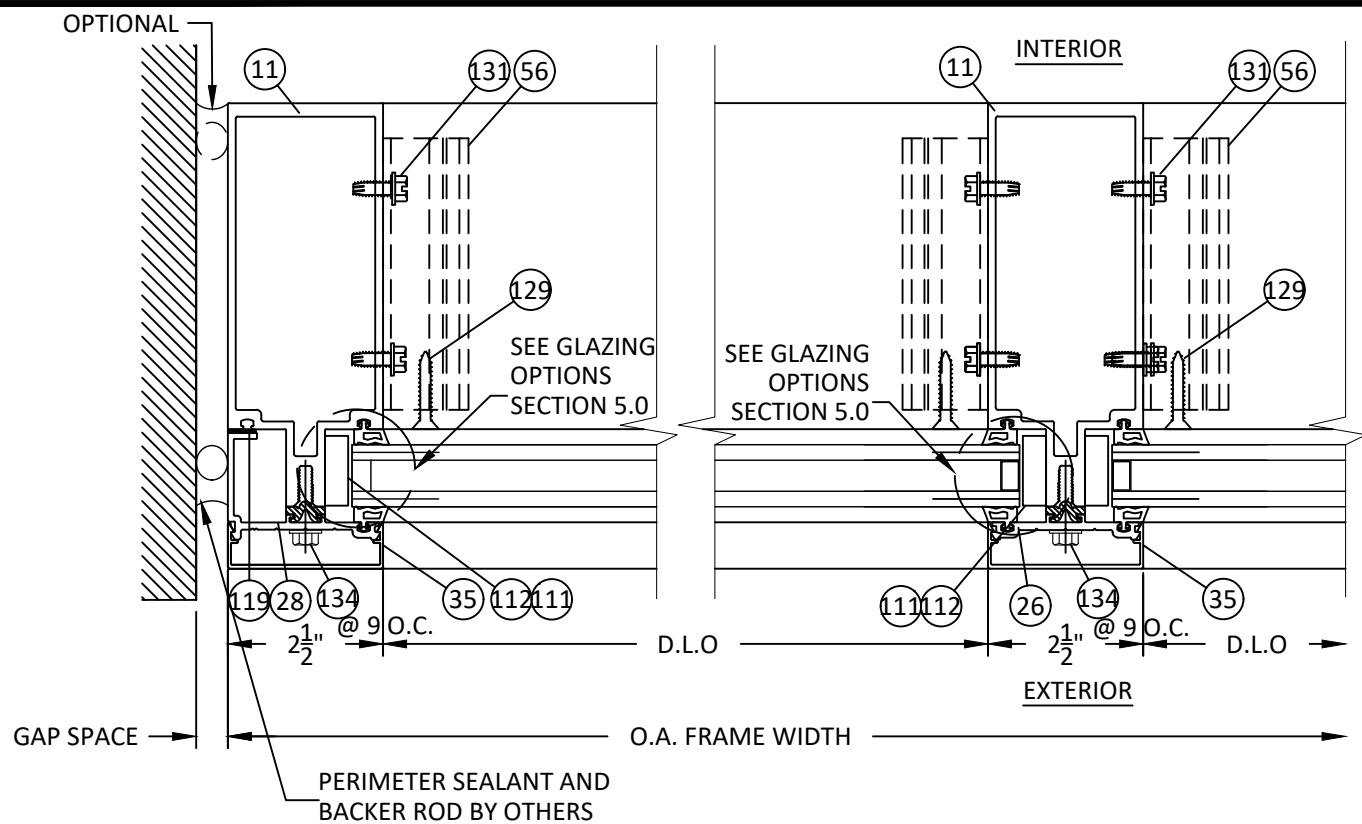
32 HORIZONTAL SECTION 4.2 7 1/2" HEAVY DUTY JAMB MULLION HEAVY DUTY TUBULAR PROFILE
