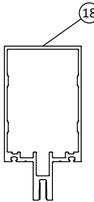
M1 VERTICAL MULLION/JAMB FOR 6" TUBULAR STANDARD
