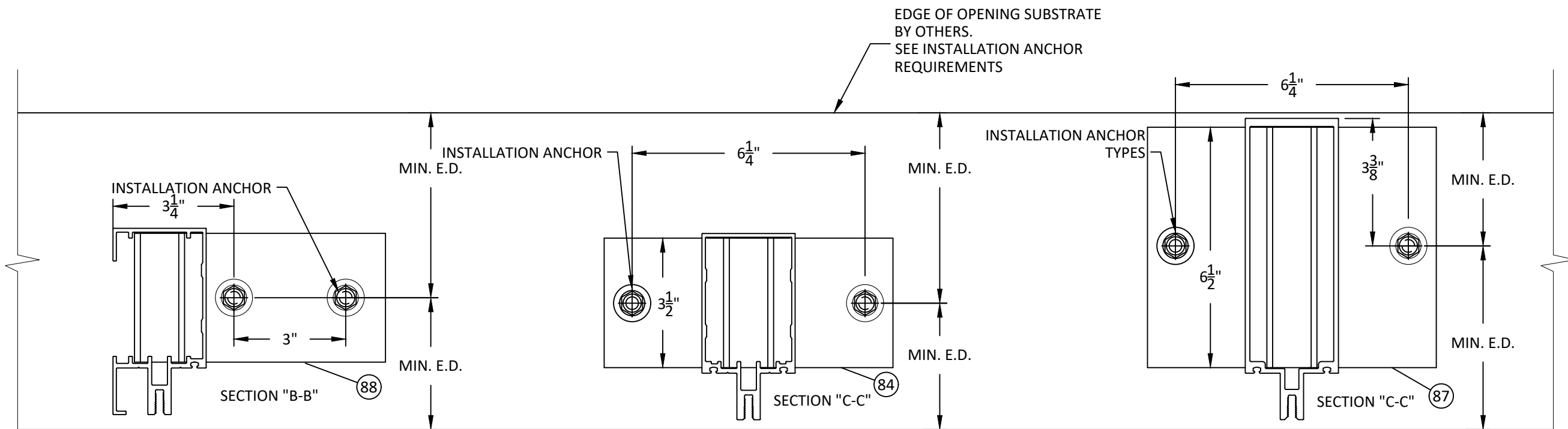
51 HORIZONTAL SECTION 6.2 F-ANCHOR CONFIG 1 6" SYSTEM
