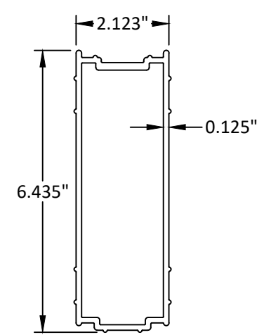
82 MULLION SPLICE SLEEVE 6063-T5
