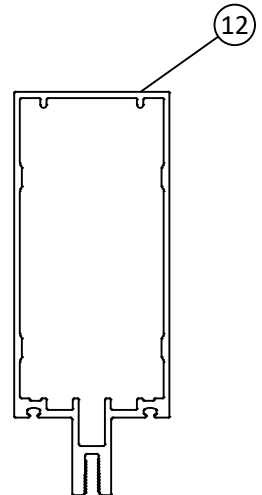
M3 VERTICAL MULLION/JAMB FOR 7-1/2" TUBULAR STANDARD
