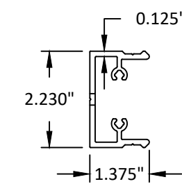
55 SHEAR BLOCK 6063-T5
