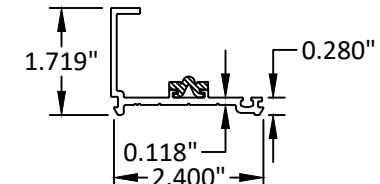
28 PRESSURE PLATE 6063-T5
