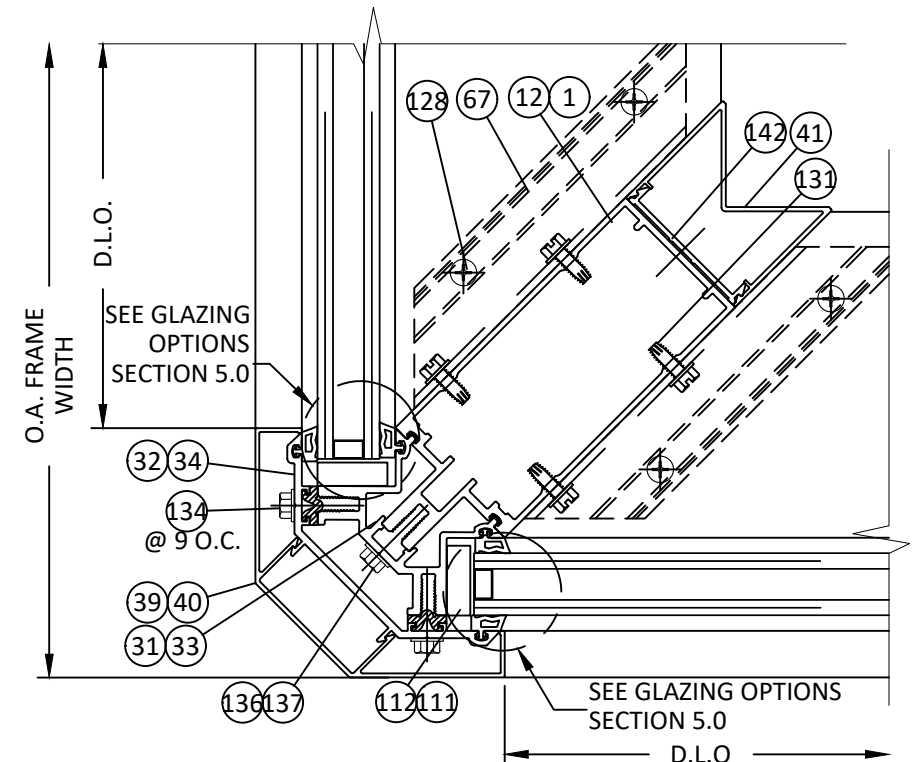
39 HORIZONTAL SECTION 4.11 90 DEG. OUTSIDE CORNER MULLION APPLICABLE FOR 7 1/2" SYSTEM
