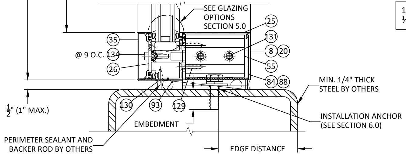
1 3.0 VERTICAL SECTION 6" SILL - STEEL STUD OPEN BACK PROFILE
