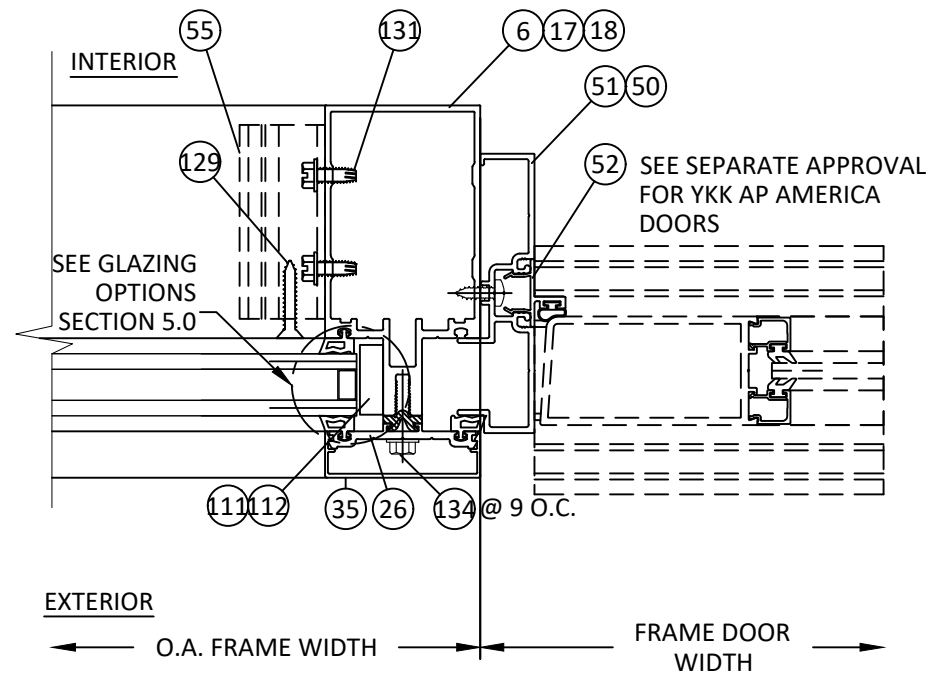
25 4.0 HORIZONTAL SECTION 6" DOOR JAMB MULLION TUBULAR PROFILE DOOR UNDER SEPARATE APPROVAL
