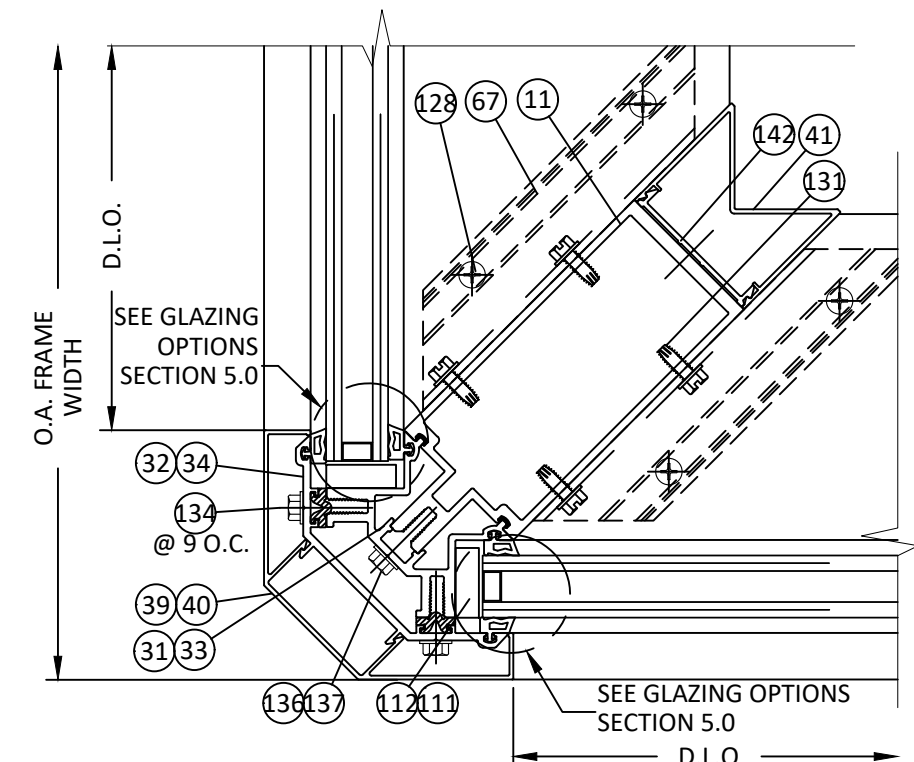
40 HORIZONTAL SECTION 4.11 90 DEG. OUTSIDE CORNER MULLION APPLICABLE FOR 7 1/2" HEAVY DUTY SYSTEM
