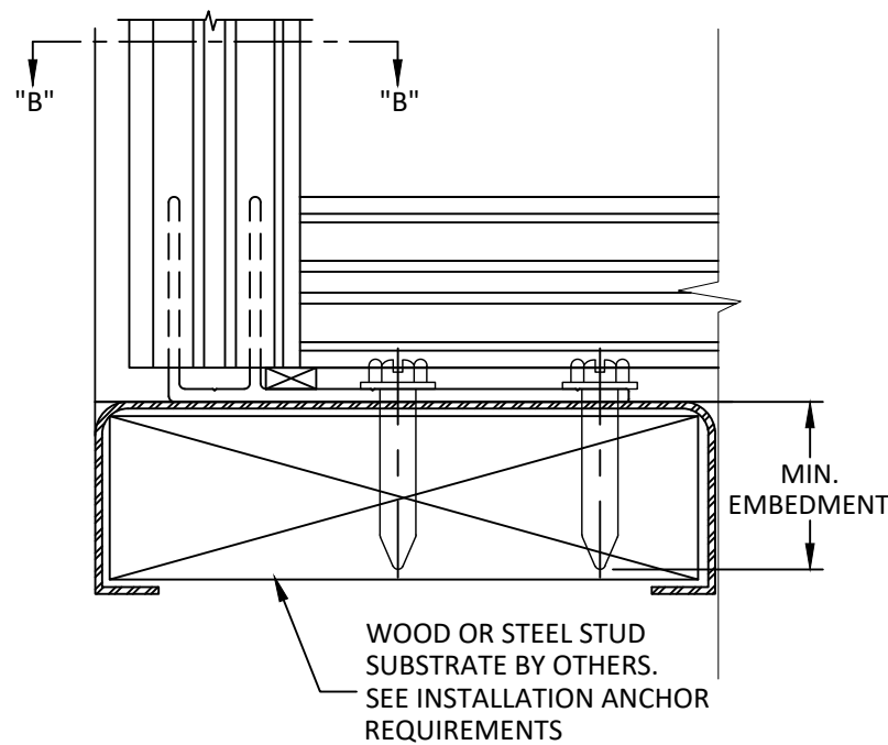
EXTERIOR VIEW F-ANCHOR (TYPICAL)
