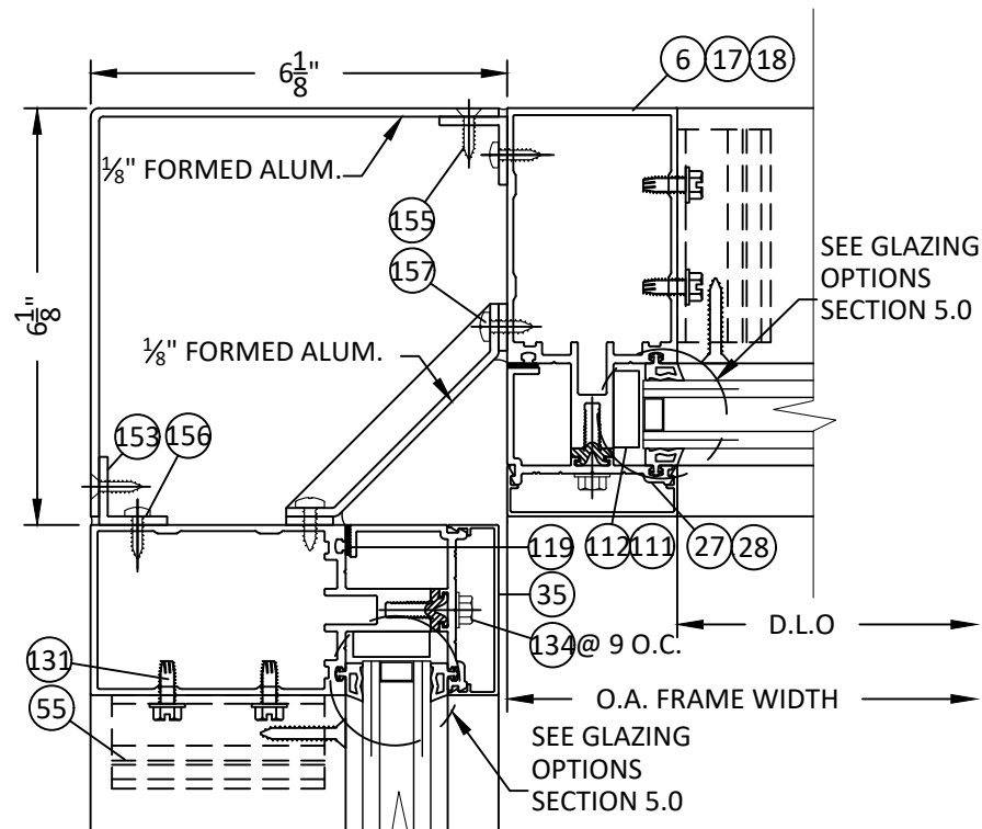
44 HORIZONTAL SECTION 4.12 90 DEG. INSIDE CORNER OPTIONAL APPLICABLE FOR 6" SYSTEM
