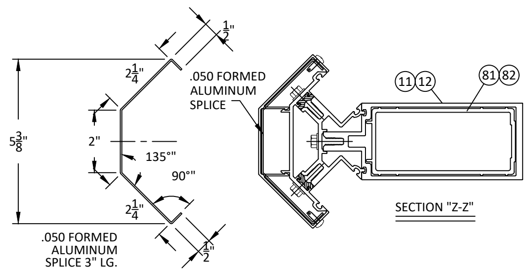
55 6.3 SPLICE SLEEVE HORIZONTAL DETAIL
