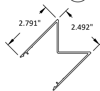
42 90 ° OUTSIDE CORNER INT. COVER 6063-T5
