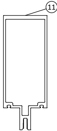
M4 VERTICAL MULLION/ JAMB FOR 7-1/2" HEAVY DUTY TUBULAR OPTION
