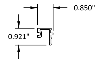
43 GLAZING ADAPTOR 6063-T5
