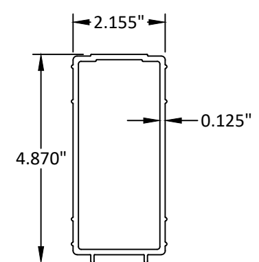
81 MULLION SPLICE SLEEVE 6063-T5
