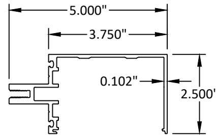
22 HORIZONTAL FOR 1" GL 6063-T5
