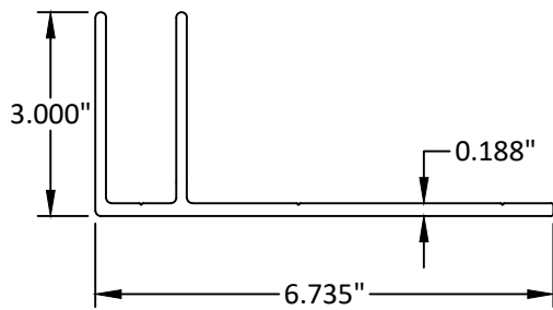
88 MULLION "F" ANCHOR 6063-T5
