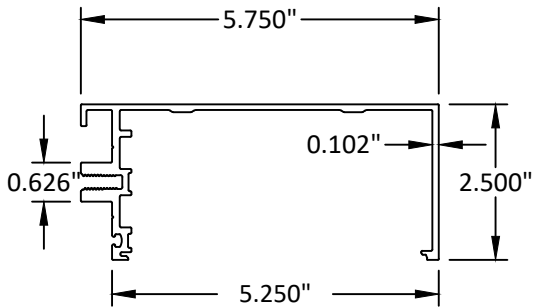
3 HEAD/ SILL FOR 1/4" GLASS 6063-T5
