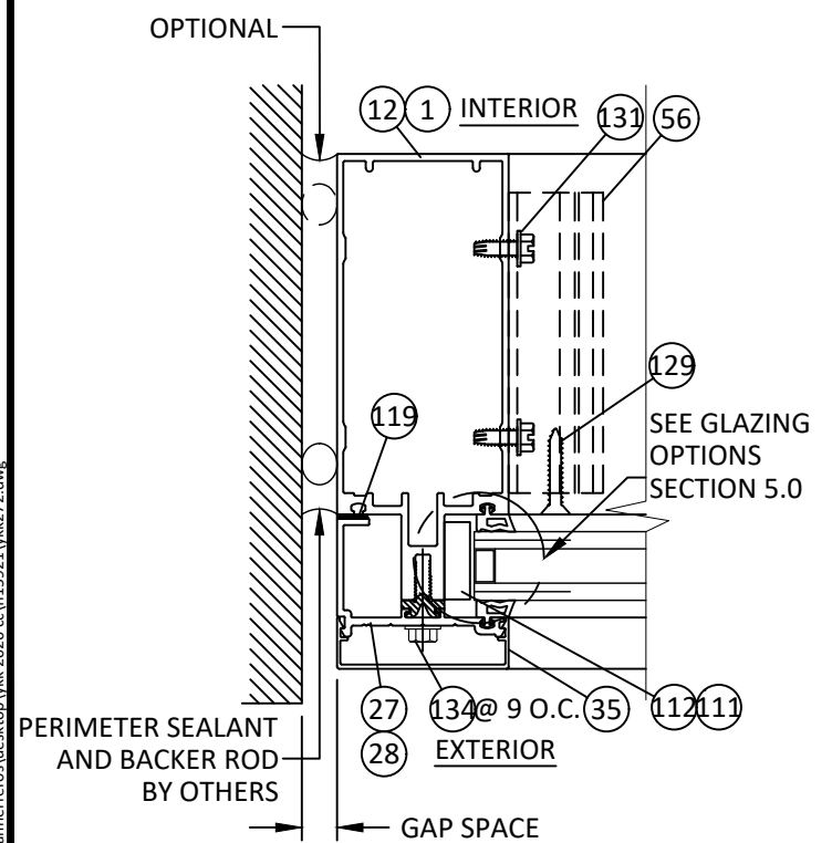
30 4.1 HORIZONTAL SECTION 7 1/2" JAMB MULLION TUBULAR PROFILE
