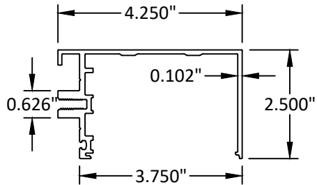
8 HEAD/ SILL FOR 1/4" GL (OPEN BACK) 6063-T5
