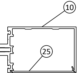
HORIZONTAL MULLION FOR 6" TUBULAR STANDARD
